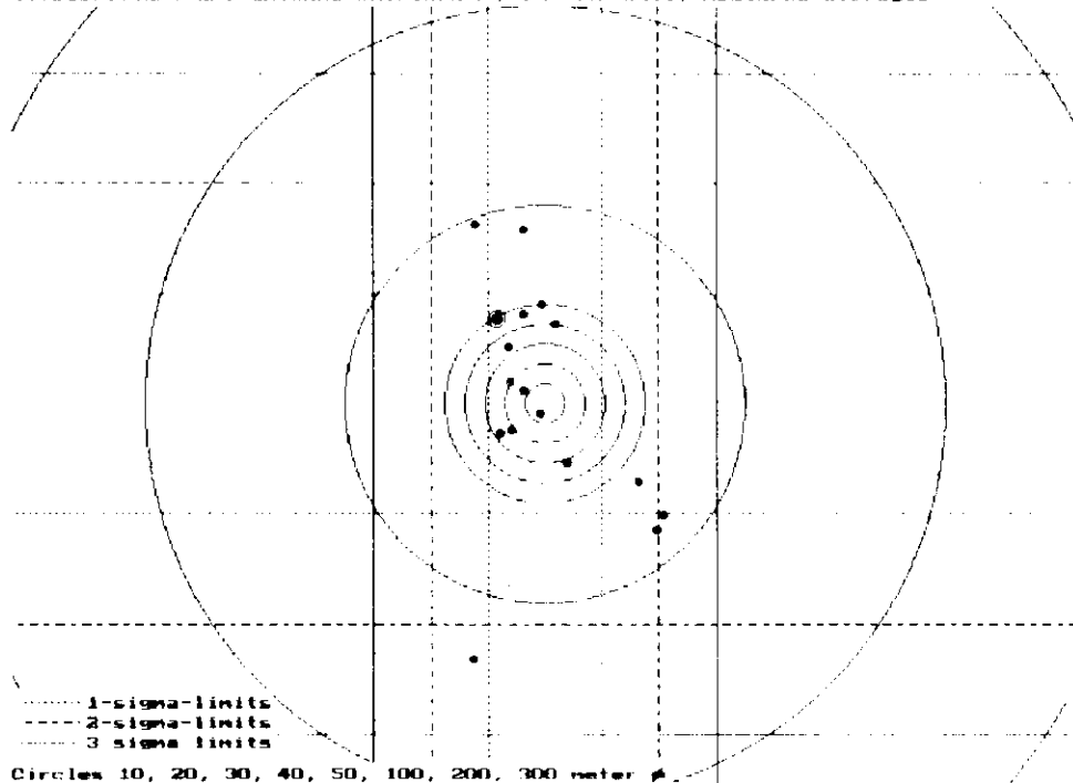
..... 1-sigma-limits ----- 2-sigma-limits ..... 3 sigma limits Circles 10, 20, 30, 40, 50, 100, 200, 300 meter # Plot C-4
