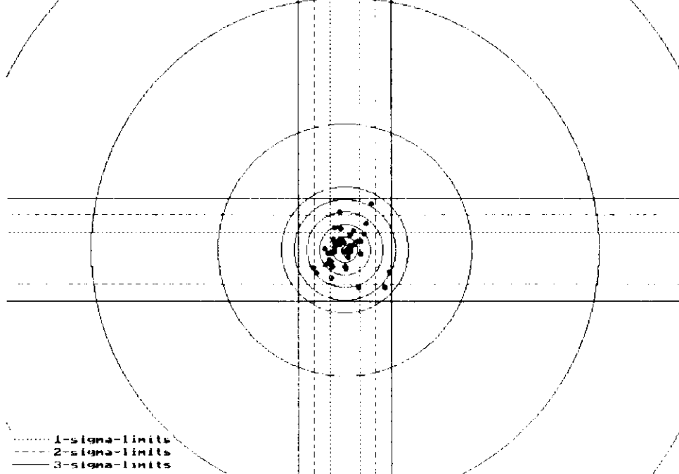
..... 1-sigma-limits ----- 2-sigma-limits ———— 3-sigma-limits Circles 10, 20, 30, 40, 50, 100, 200, 300 meter # Plot B-4
