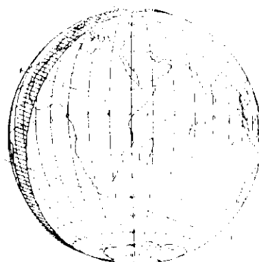
ZC 2025 by Jupiter 93 Nov 29
