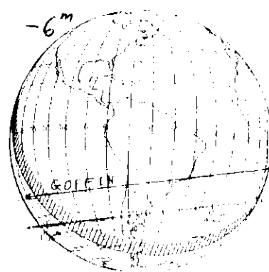
SAO 131238 by Artemis Dec 11
