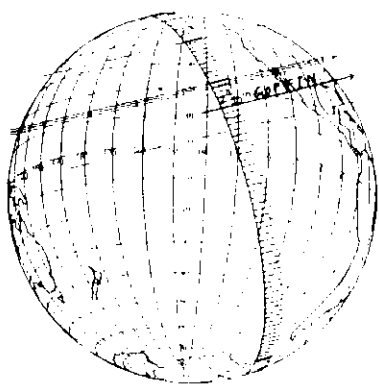
SAO 164056 by Fortuna 93 Nov 23
