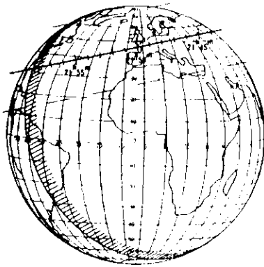
SAO 110007 by Glauke 93 Nov 20
