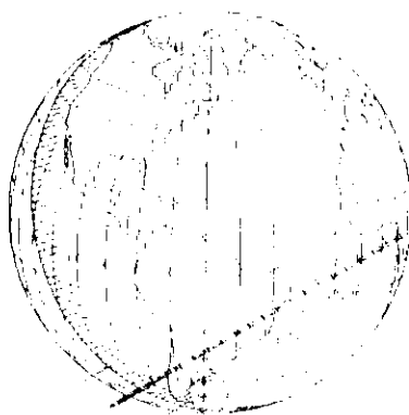
ZC 466 by Victoria 93 Dec 11
