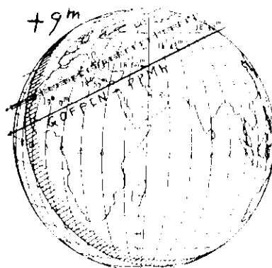
SAO 110612 by Gyptis Nov 27
