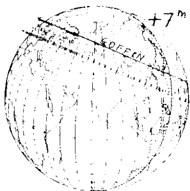
BD +24° 1499 by Vibilia Nov 30
