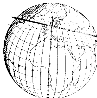
SAO 78468 by Vibilia 93 Dec 31
