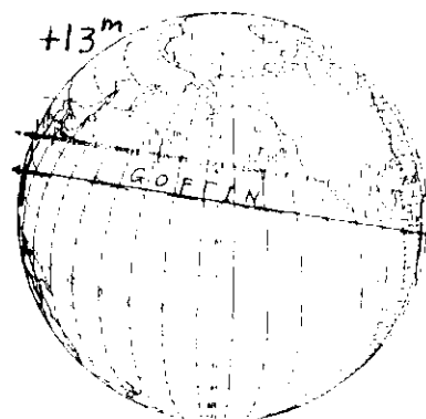
SAO 115514 by Klotho 93 Dec 22
