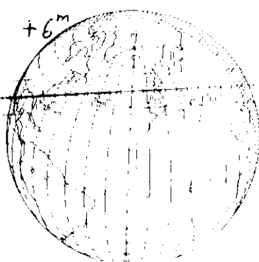
BD +19° 750 by Aurelia Dec 13
